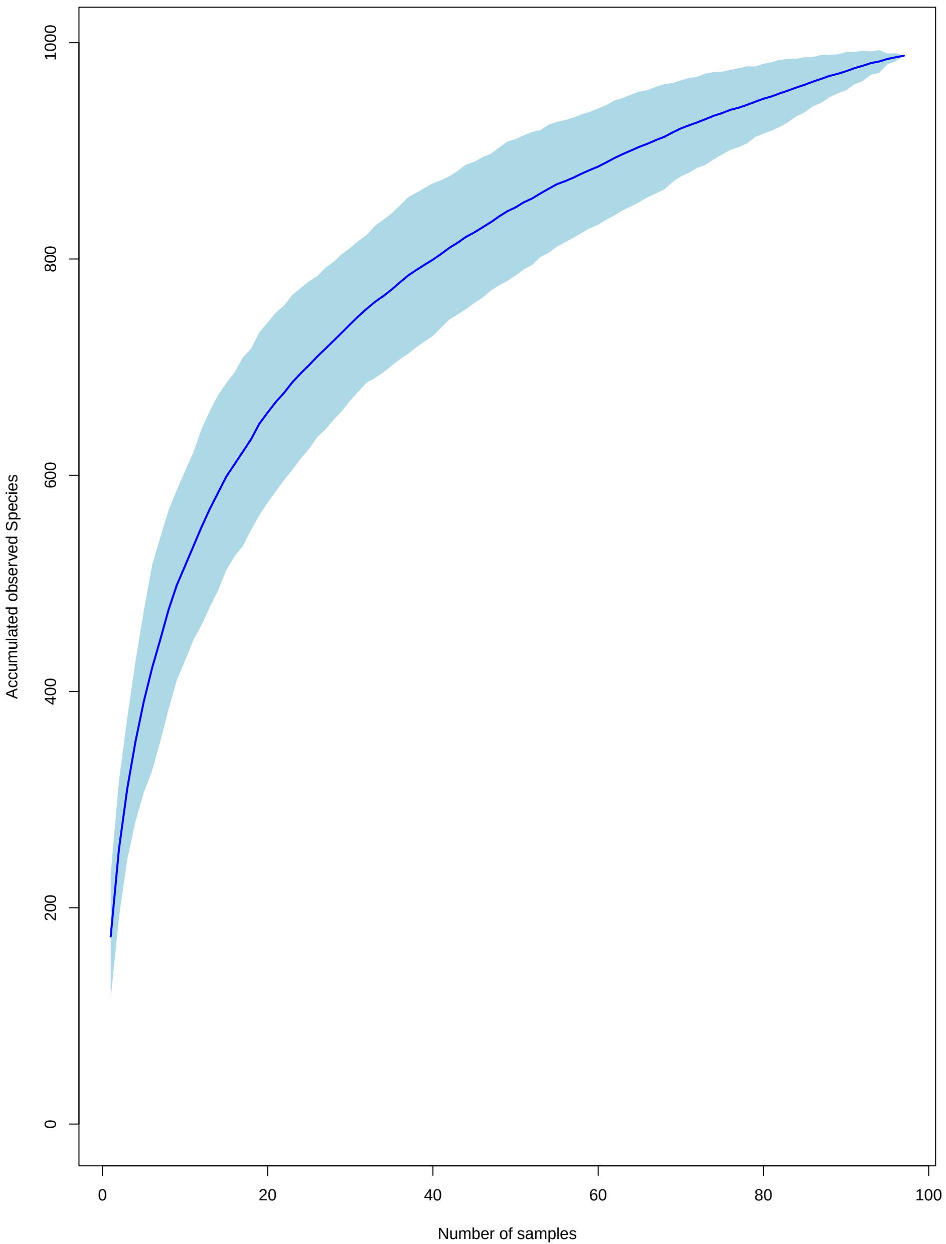
Species Accumulation Curve
